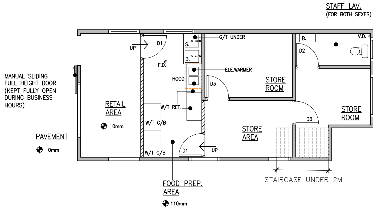
LAYOUT PLAN SCALE:1:75
