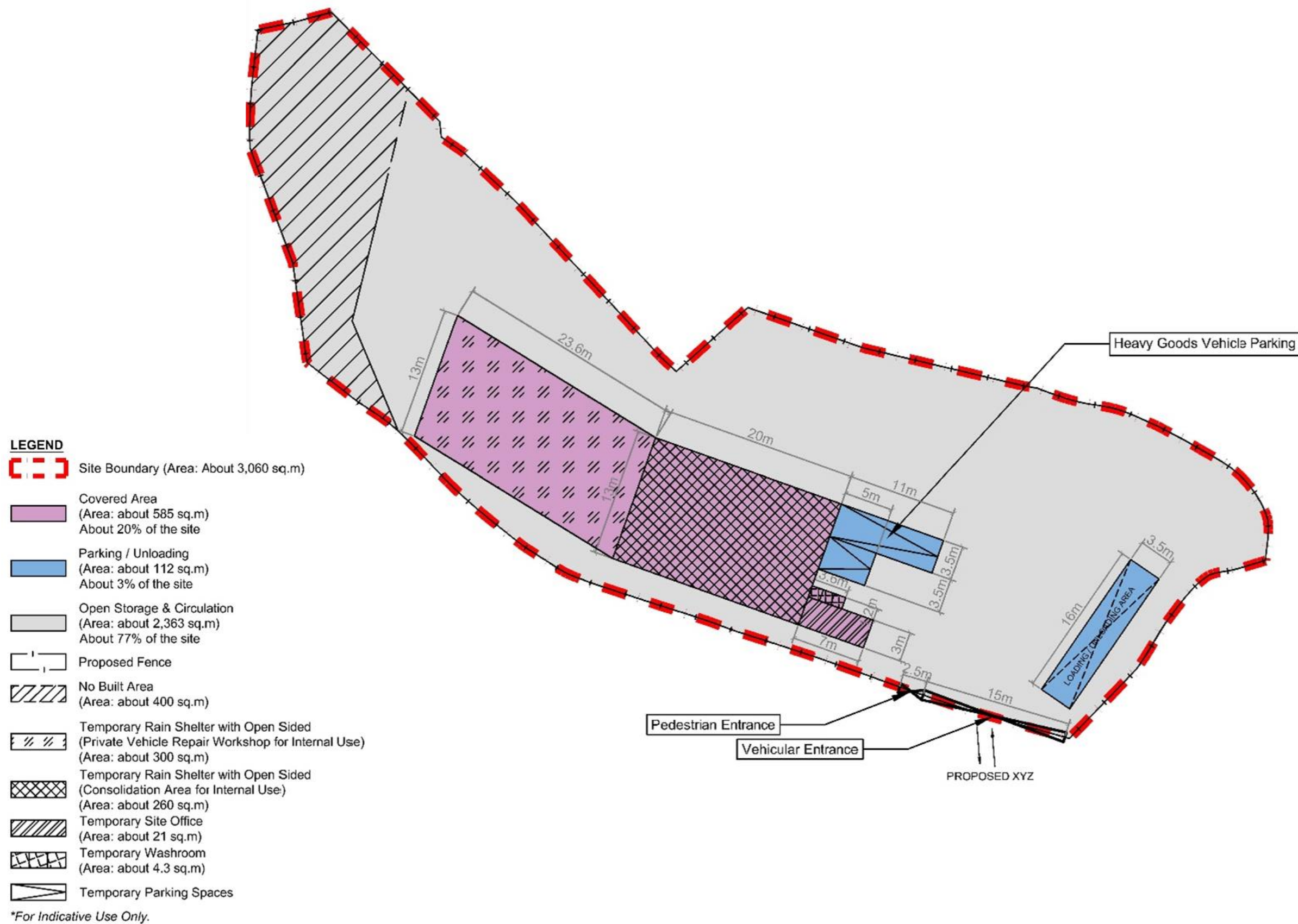
Figure 1.3 Layout Plan
