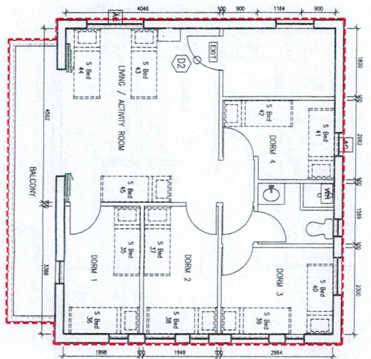
Section C (1/F) - Layout Plan Scale: 1:100
