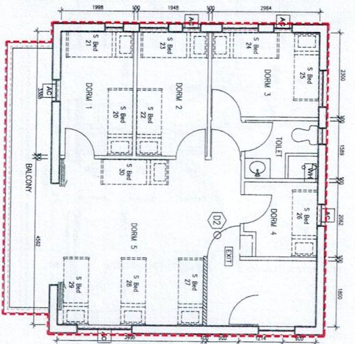
Section D (2/F) - Layout Plan Scale 1:100
