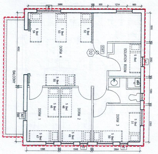
Section C (2/F) - Layout Plan Scale: 1:100
