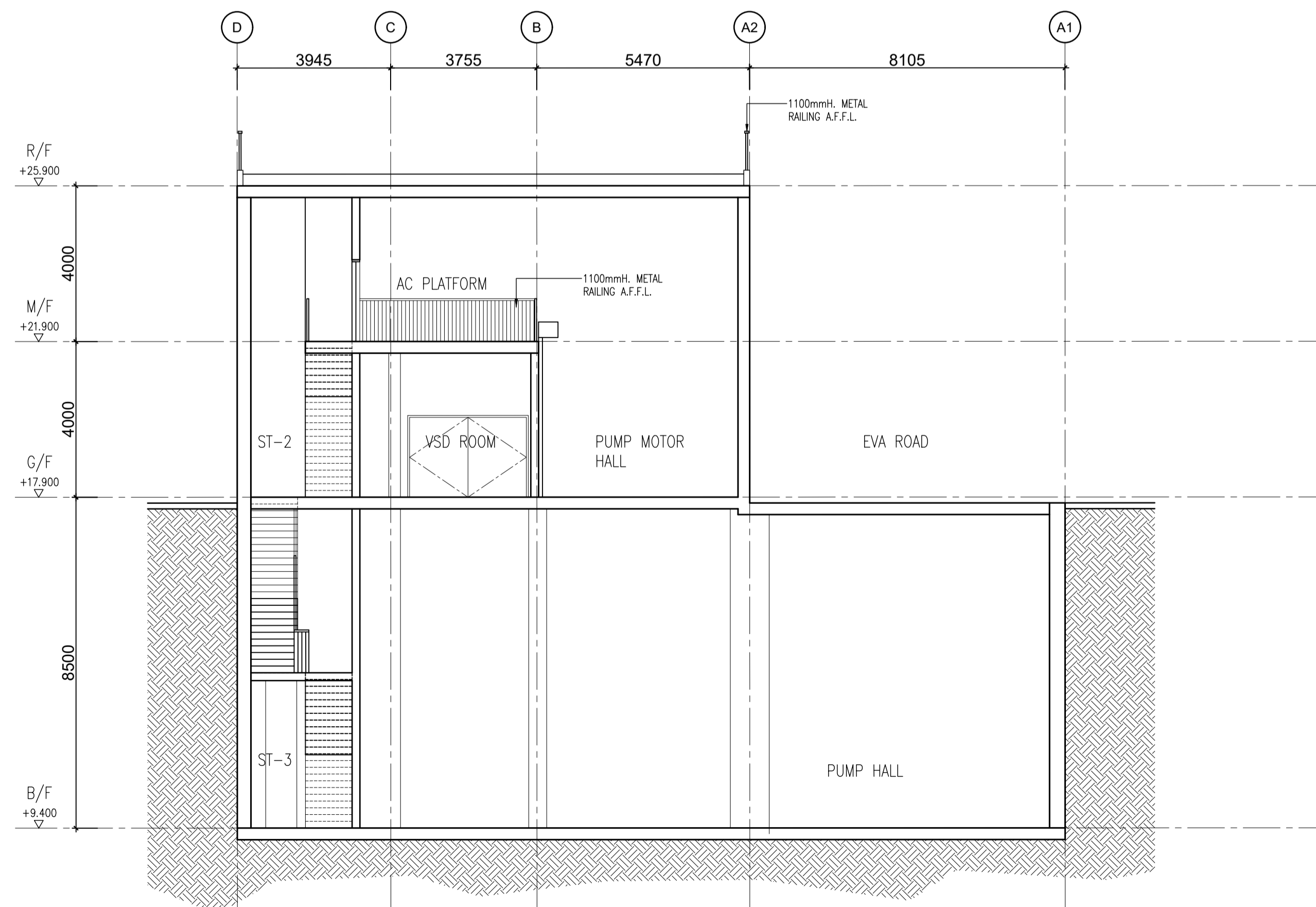
2 SECTION B SCALE 1:100@A1
