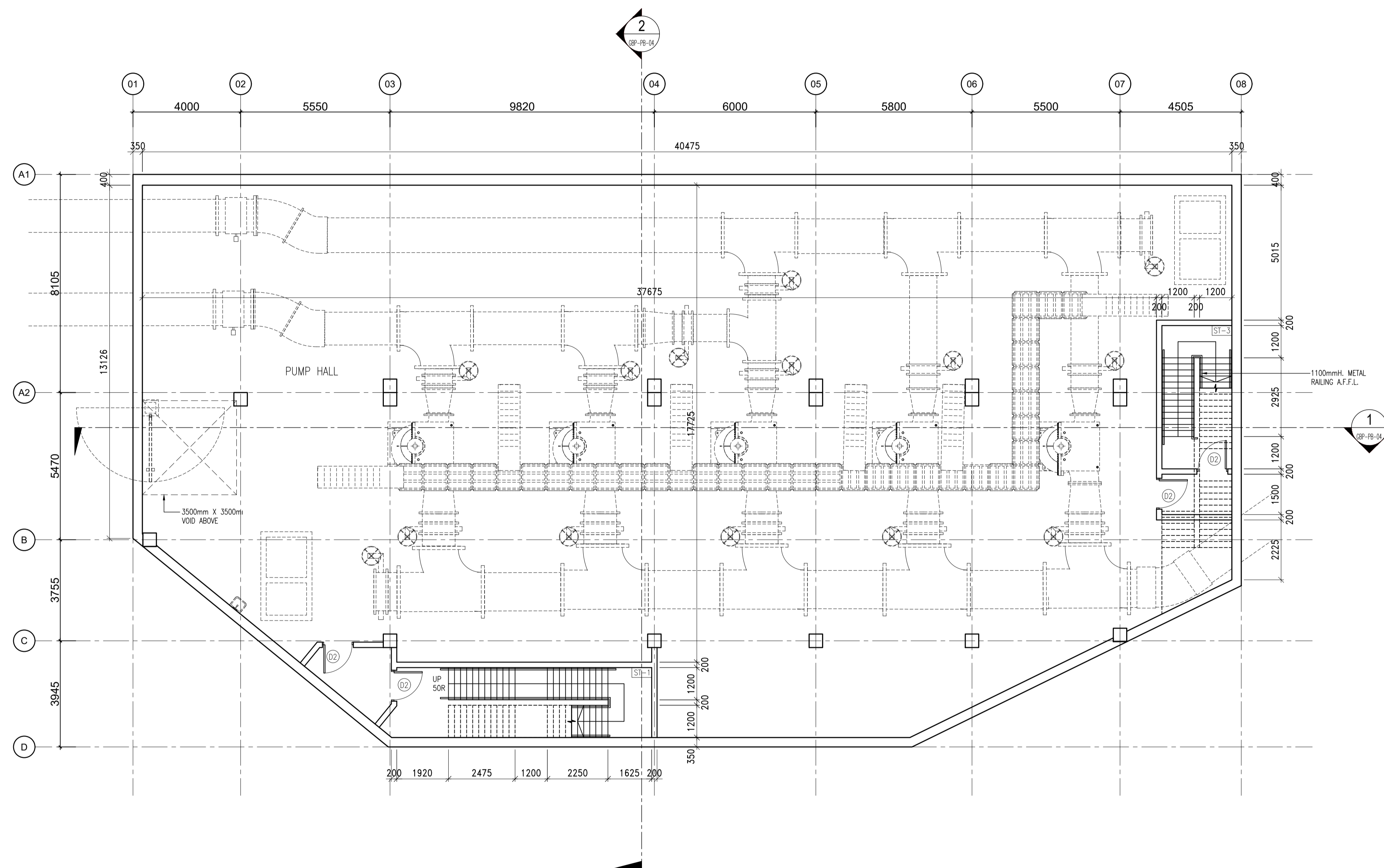
1 PUMP BUILDING BASEMENT FLOOR PLAN SCALE 1:100@A1
