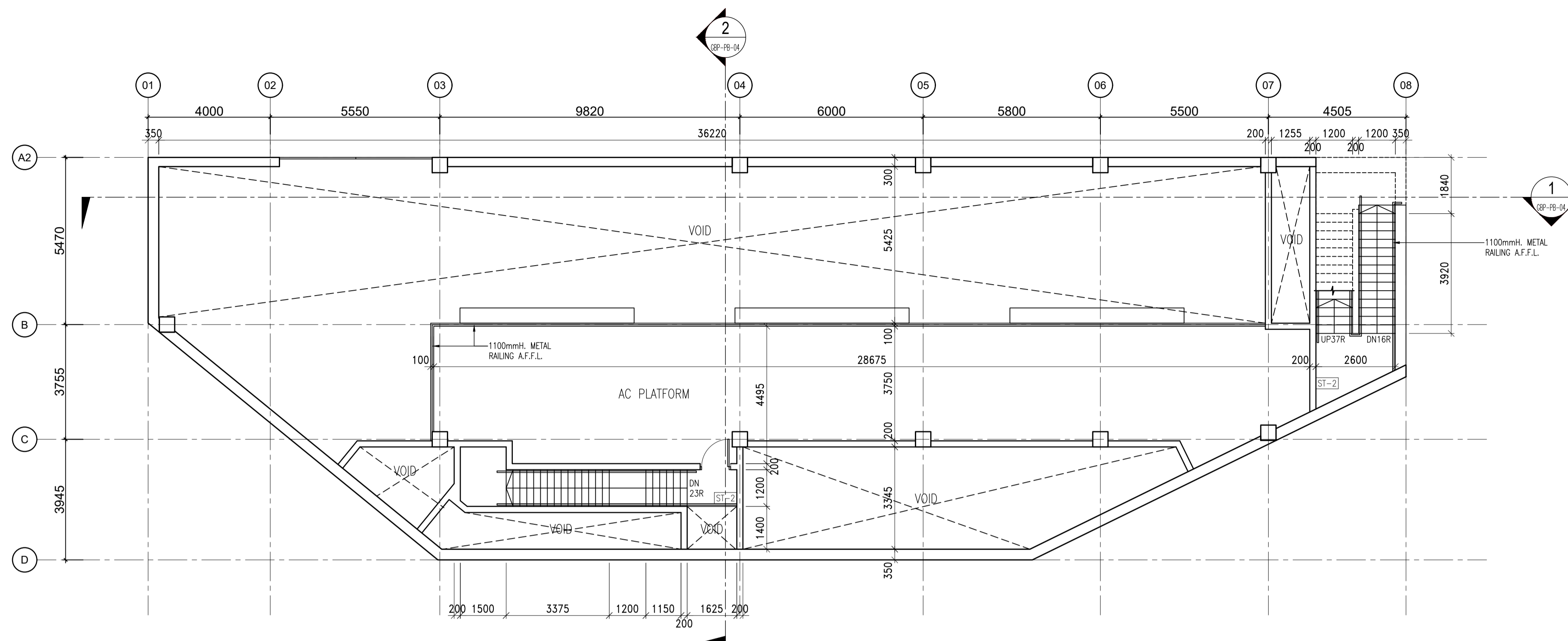
1 PUMP BUILDING MEZZANINE FLOOR PLAN - SCALE 1:100@A1
