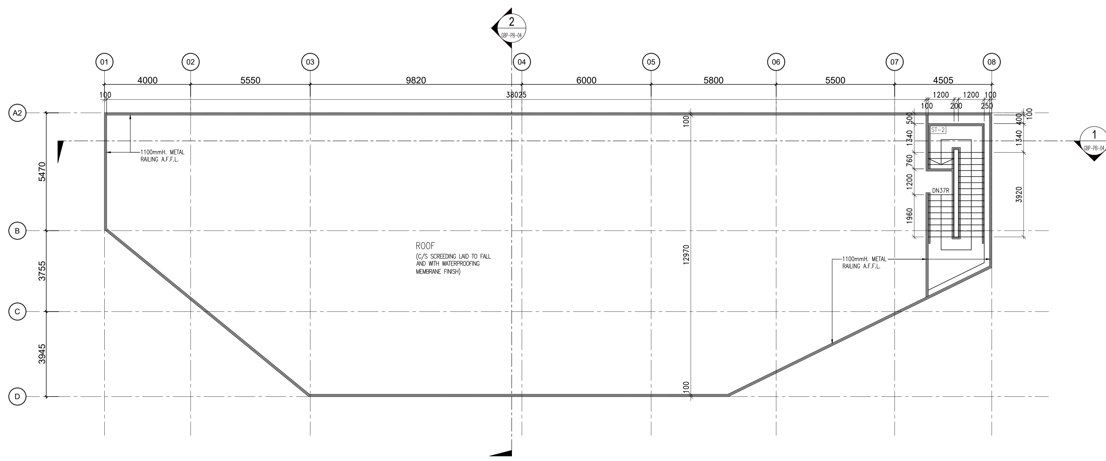
2 PUMP BUILDING ROOF PLAN - SCALE 1:100@A1
