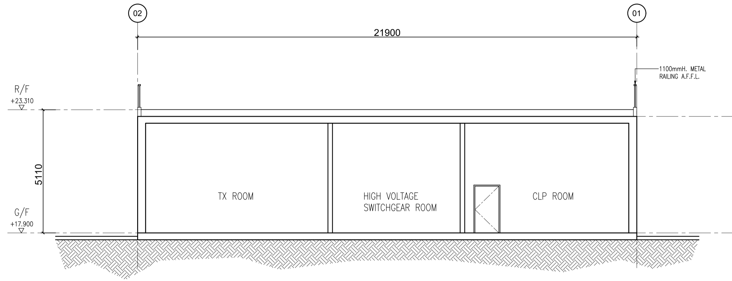
1 SECTION A SCALE 1:100@A1
