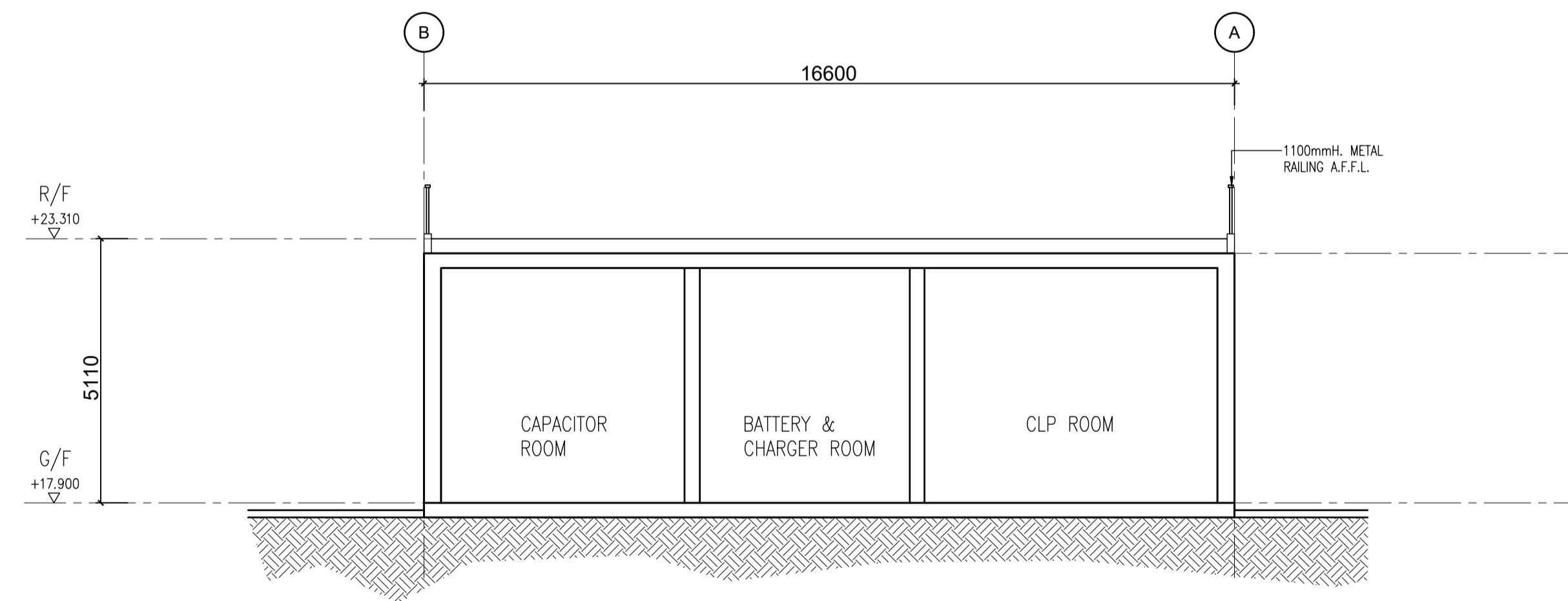
2 SECTION B SCALE 1:100@A1
