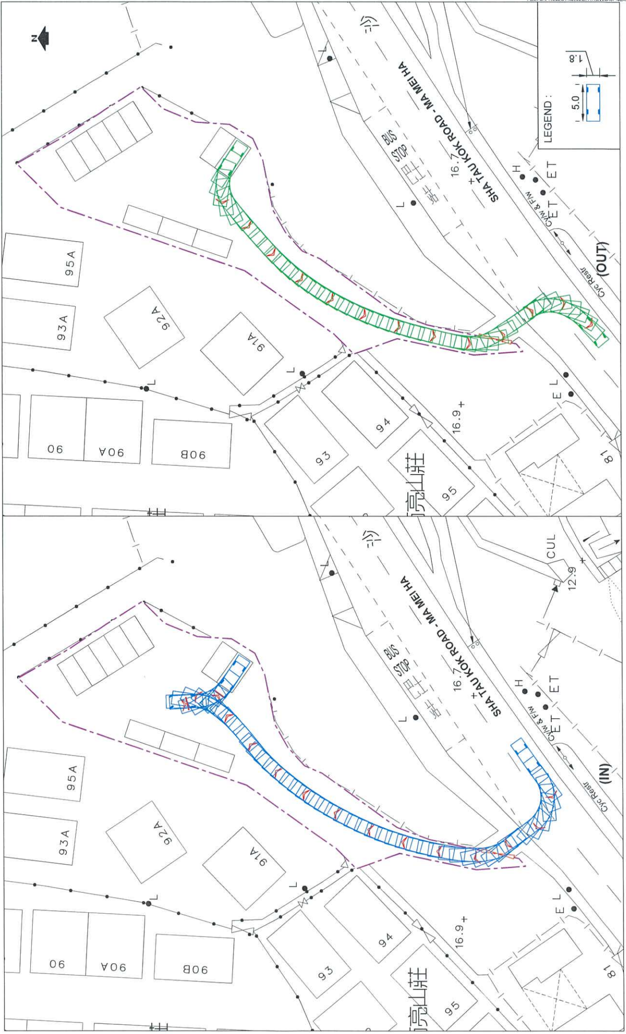
SWEPT PATH ANALYSIS - PC (TO / FROM SHA TAU KOK ROAD SOUTHBOUND) (SCALE 1:500 @ A4)
