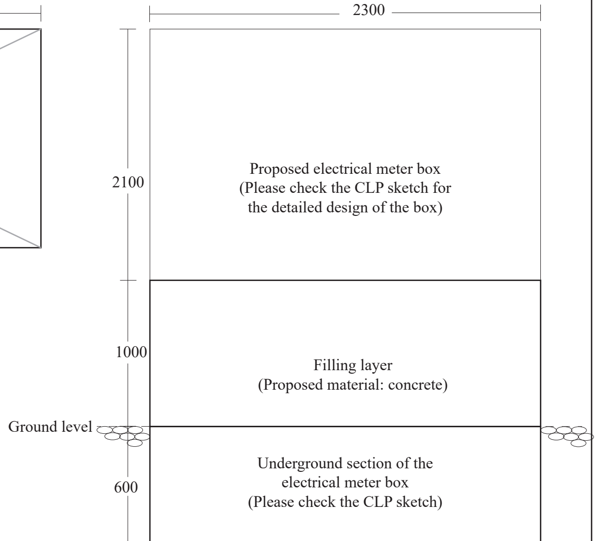
Site sectional plan with reference to ground level
