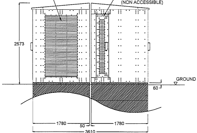
LEFT VIEW
