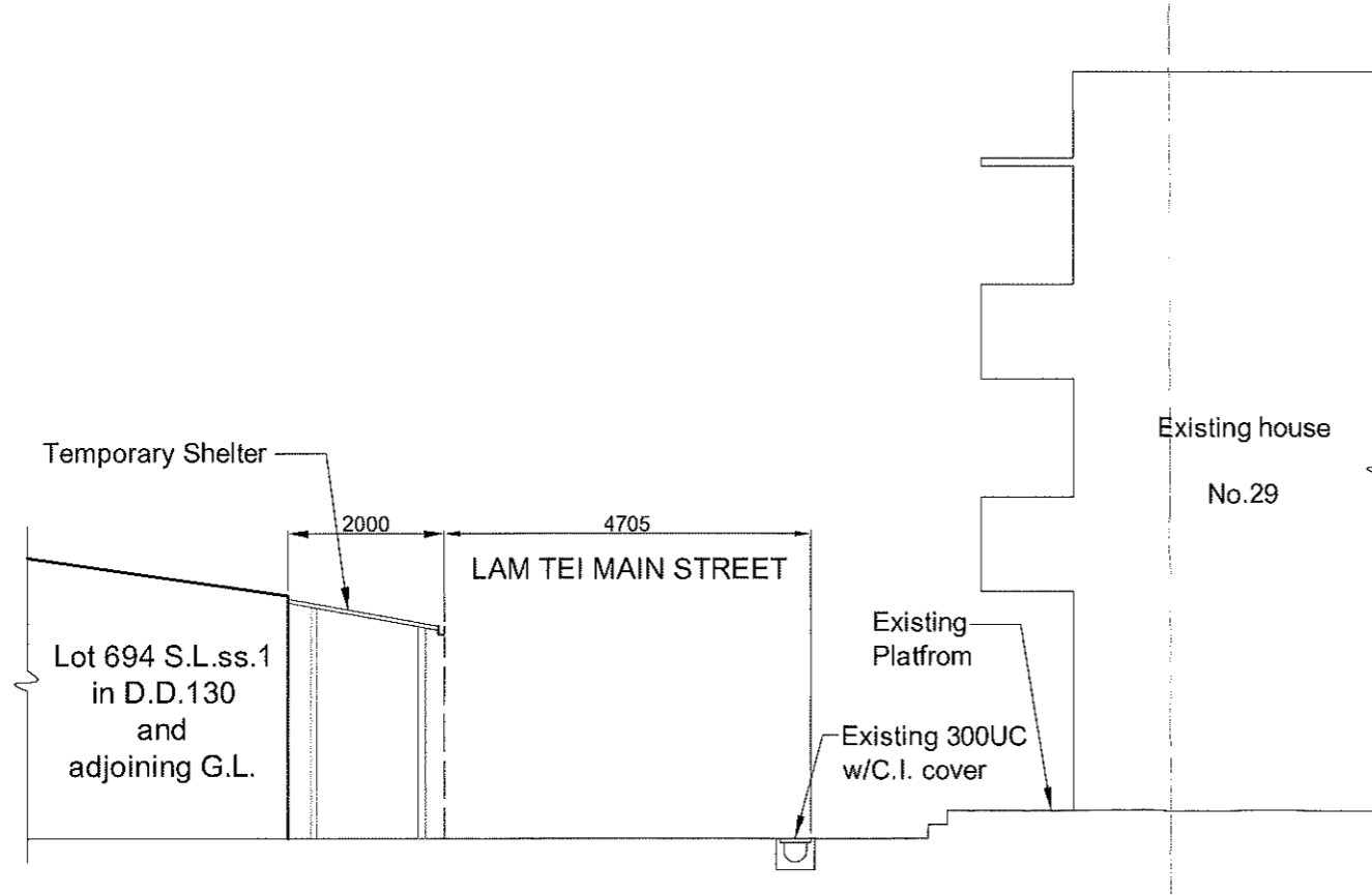
Section B - B (1:100)
