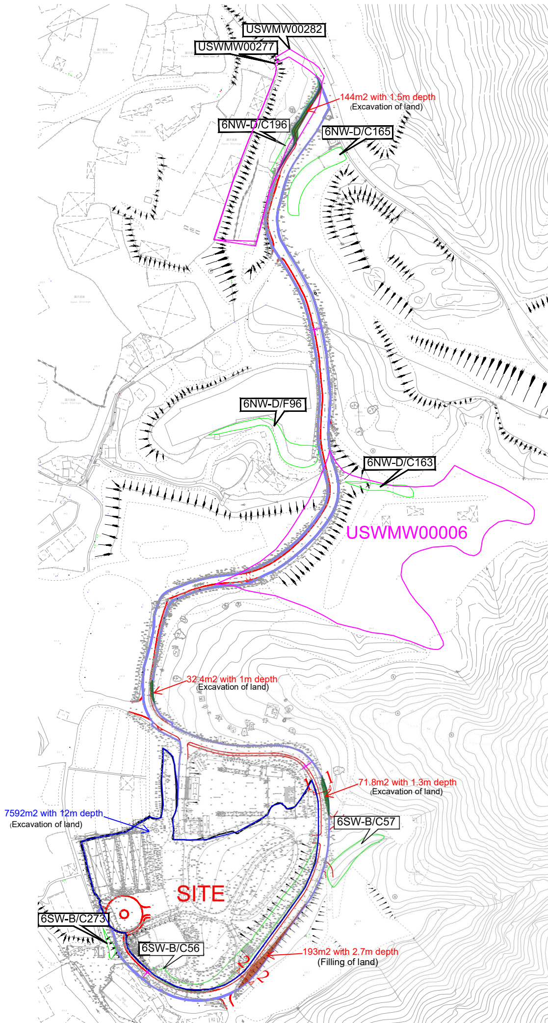
Excavation and Landfilling Plan
