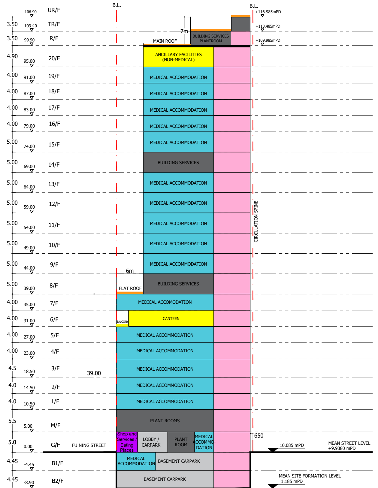
DIAGRAMMATIC SECTION
