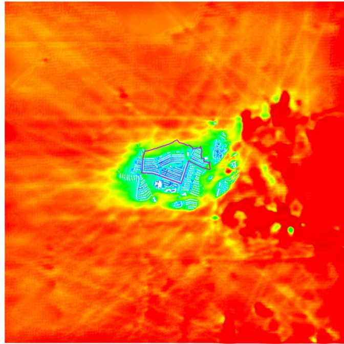
Figure 41 Annual Weighted Average VR Contour Plot of Whole Domain at Pedestrian Level for Baseline Scheme
