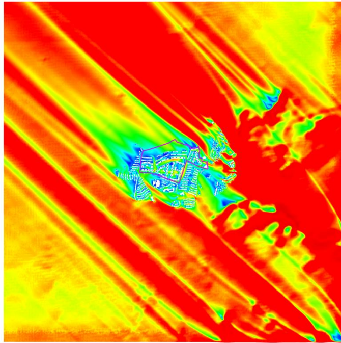
Figure 23 VR Contour Plot of Whole Domain at Pedestrian Level under SE Wind for Proposed Scheme
