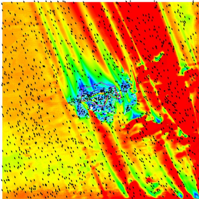
Figure 28 VR Vector Plot of Whole Domain at Pedestrian Level under SSE Wind for Proposed Scheme
