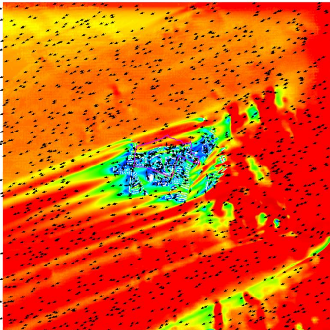
Figure 12 VR Vector Plot of Whole Domain at Pedestrian Level under ENE Wind for Proposed Scheme
