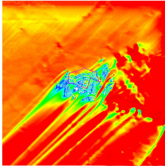
Figure 7 VR Contour Plot of Whole Domain at Pedestrian Level under NE Wind for Proposed Scheme
