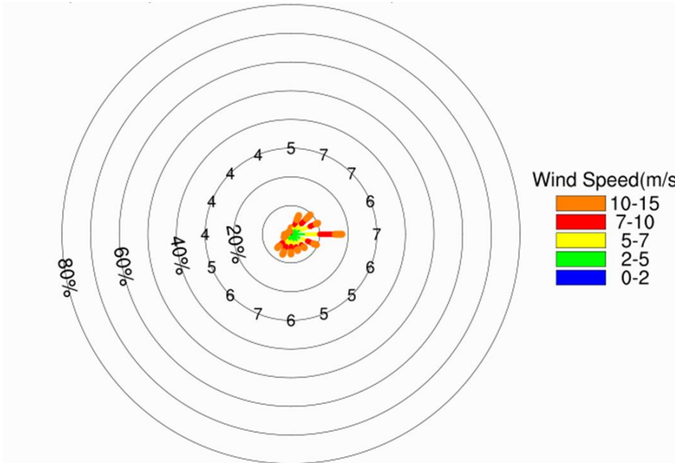
Figure 3.2: Annual Wind Rose at 500m – Grid (X055, Y080)
