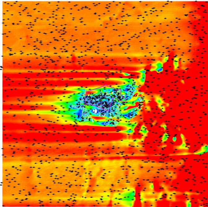
Figure 14 VR Vector Plot of Whole Domain at Pedestrian Level under E Wind for Baseline Scheme
