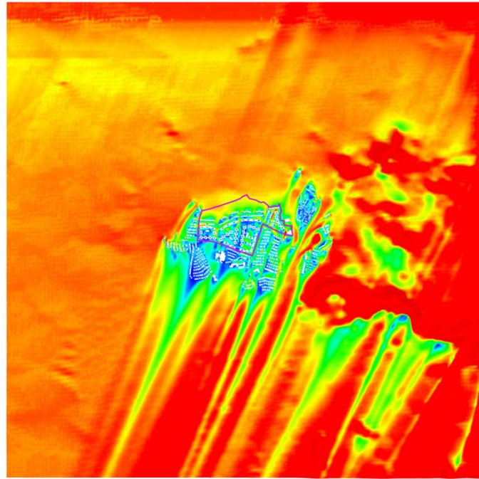
Figure 3 VR Contour Plot of Whole Domain at Pedestrian Level under NNE Wind for Proposed Scheme
