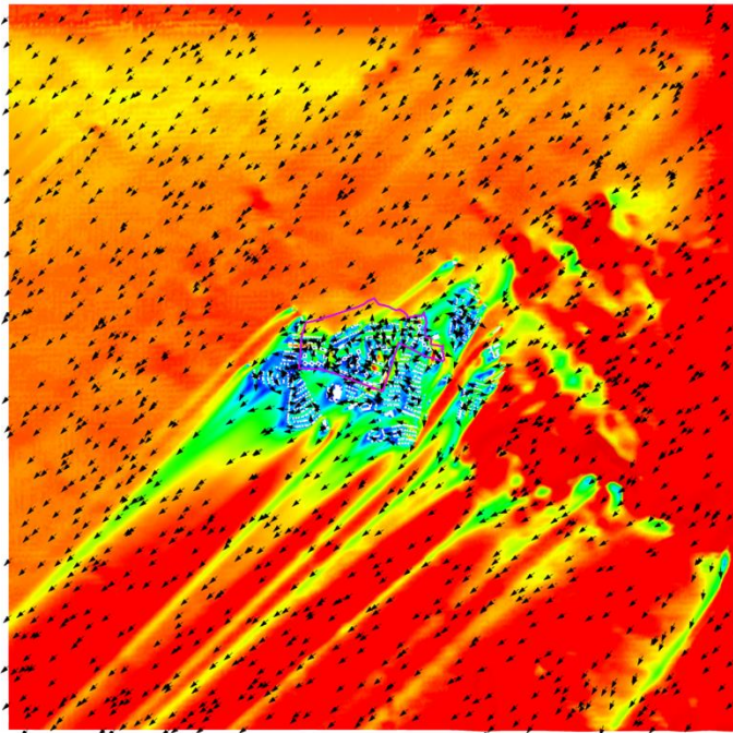
Figure 8 VR Vector Plot of Whole Domain at Pedestrian Level under NE Wind for Proposed Scheme
