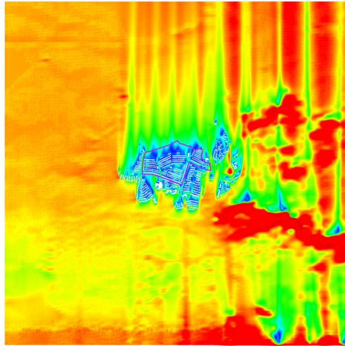
Figure 29 VR Contour Plot of Whole Domain at Pedestrian Level under S Wind for Baseline Scheme
