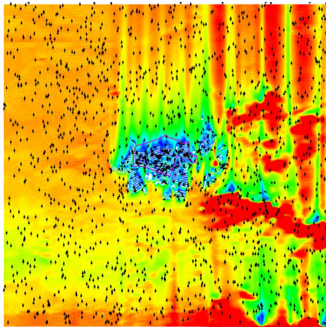
Figure 30 VR Vector Plot of Whole Domain at Pedestrian Level under S Wind for Baseline Scheme
