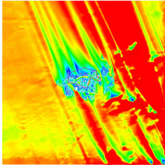
Figure 27 VR Contour Plot of Whole Domain at Pedestrian Level under SSE Wind for Proposed Scheme
