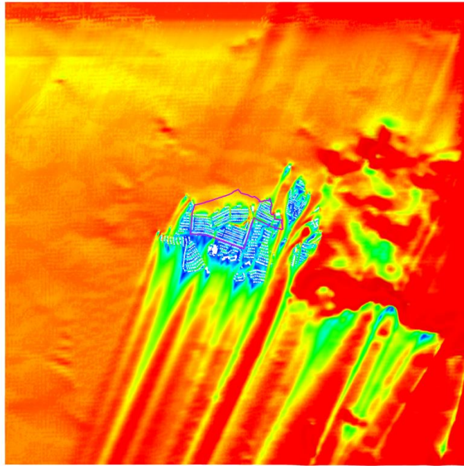
Figure 1 VR Contour Plot of Whole Domain at Pedestrian Level under NNE Wind for Baseline Scheme
