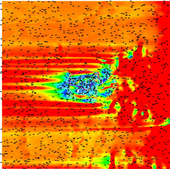
Figure 16 VR Vector Plot of Whole Domain at Pedestrian Level under E Wind for Proposed Scheme
