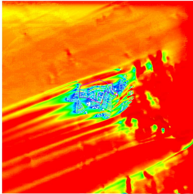
Figure 11 VR Contour Plot of Whole Domain at Pedestrian Level under ENE Wind for Proposed Scheme
