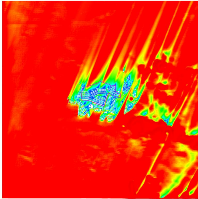
Figure 33 VR Contour Plot of Whole Domain at Pedestrian Level under SSW Wind for Baseline Scheme
