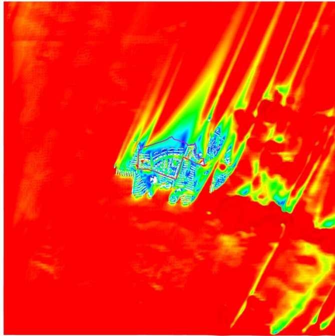
Figure 35 VR Contour Plot of Whole Domain at Pedestrian Level under SSW Wind for Proposed Scheme
