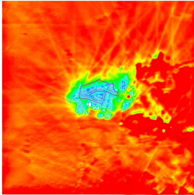
Figure 43 Summer Weighted Average VR Contour Plot of Whole Domain at Pedestrian Level for Baseline Scheme
