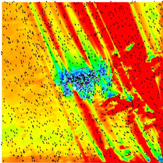
Figure 26 VR Vector Plot of Whole Domain at Pedestrian Level under SSE Wind for Baseline Scheme
