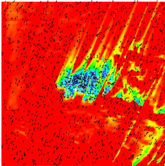
Figure 34 VR Vector Plot of Whole Domain at Pedestrian Level under SSW Wind for Baseline Scheme
