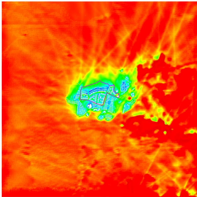
Figure 44 Summer Weighted Average VR Contour Plot of Whole Domain at Pedestrian Level for Proposed Scheme
