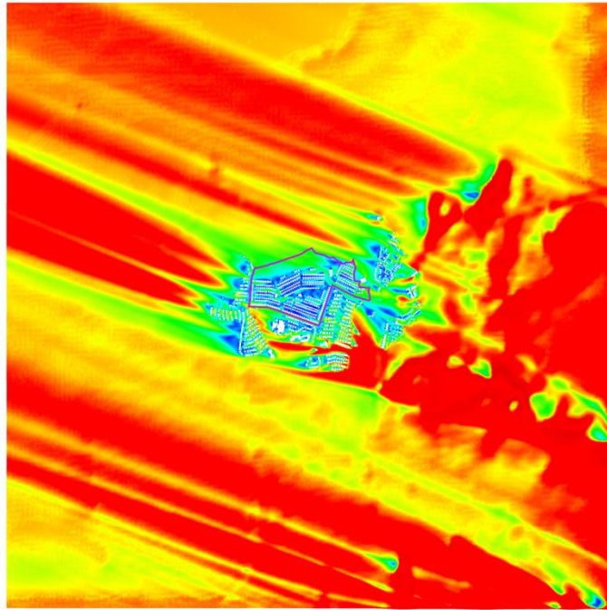
Figure 17 VR Contour Plot of Whole Domain at Pedestrian Level under ESE Wind for Baseline Scheme
