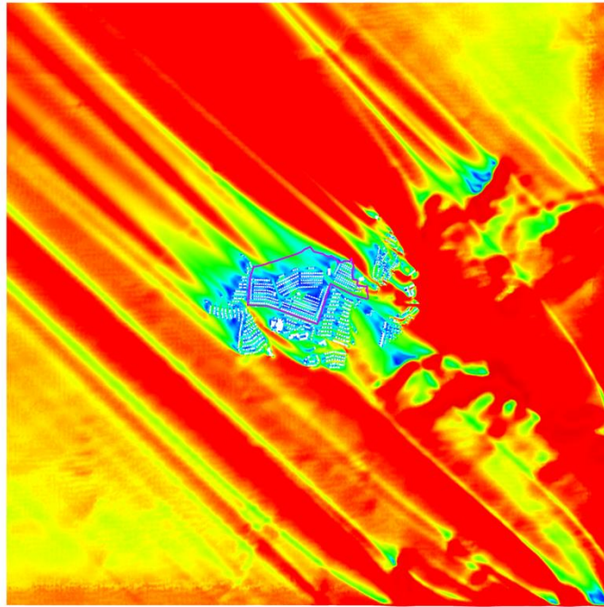
Figure 21 VR Contour Plot of Whole Domain at Pedestrian Level under SE Wind for Baseline Scheme
