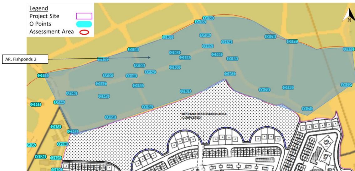
Figure 5.17: Location of the Focus Areas within the Assessment Area (North)
