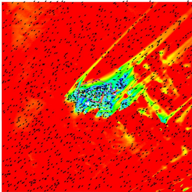
Figure 40 VR Vector Plot of Whole Domain at Pedestrian Level under SW Wind for Proposed Scheme
