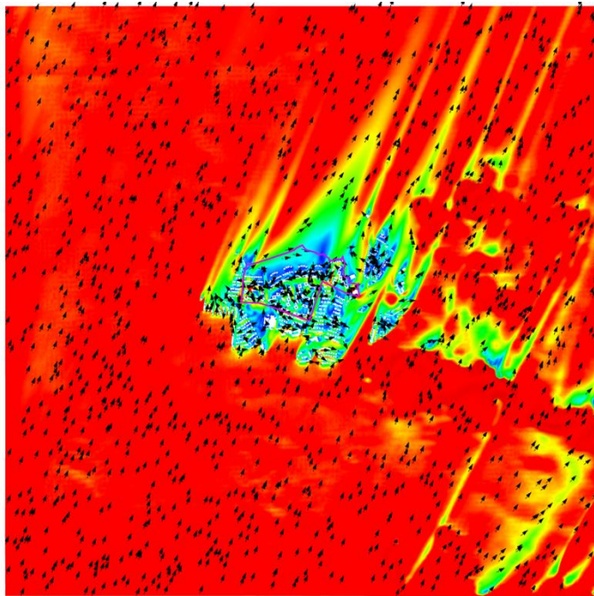
Figure 36 VR Vector Plot of Whole Domain at Pedestrian Level under SSW Wind for Proposed Scheme
