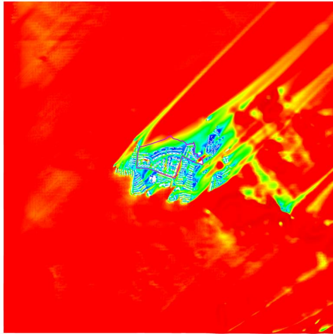
Figure 39 VR Contour Plot of Whole Domain at Pedestrian Level under SW Wind for Proposed Scheme
