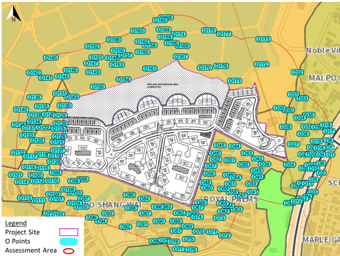
Figure 5.6: Demarcation of the Overall (O) Test Points in Proposed Scheme
