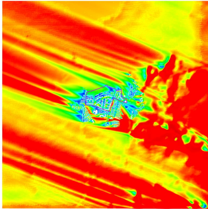
Figure 19 VR Contour Plot of Whole Domain at Pedestrian Level under ESE Wind for Proposed Scheme
