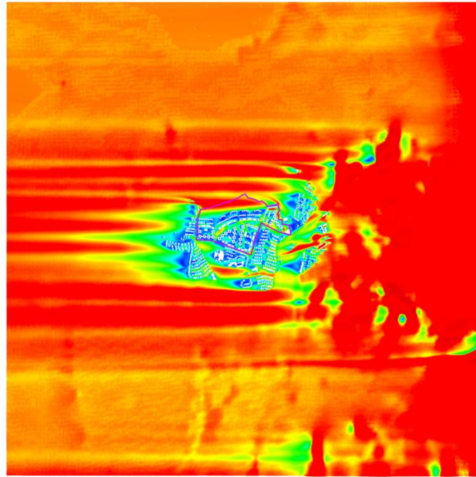
Figure 15 VR Contour Plot of Whole Domain at Pedestrian Level under E Wind for Proposed Scheme
