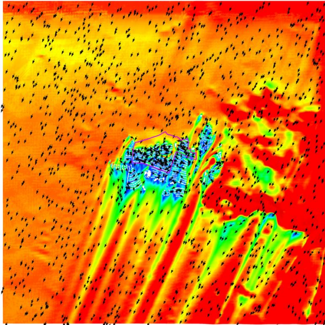
Figure 2 VR Vector Plot of Whole Domain at Pedestrian Level under NNE Wind for Baseline Scheme
