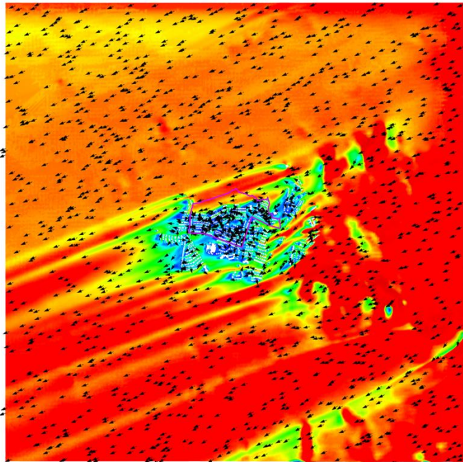
Figure 10 VR Vector Plot of Whole Domain at Pedestrian Level under ENE Wind for Baseline Scheme
