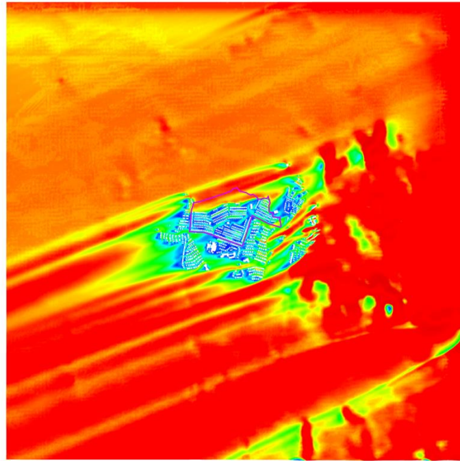
Figure 9 VR Contour Plot of Whole Domain at Pedestrian Level under ENE Wind for Baseline Scheme
