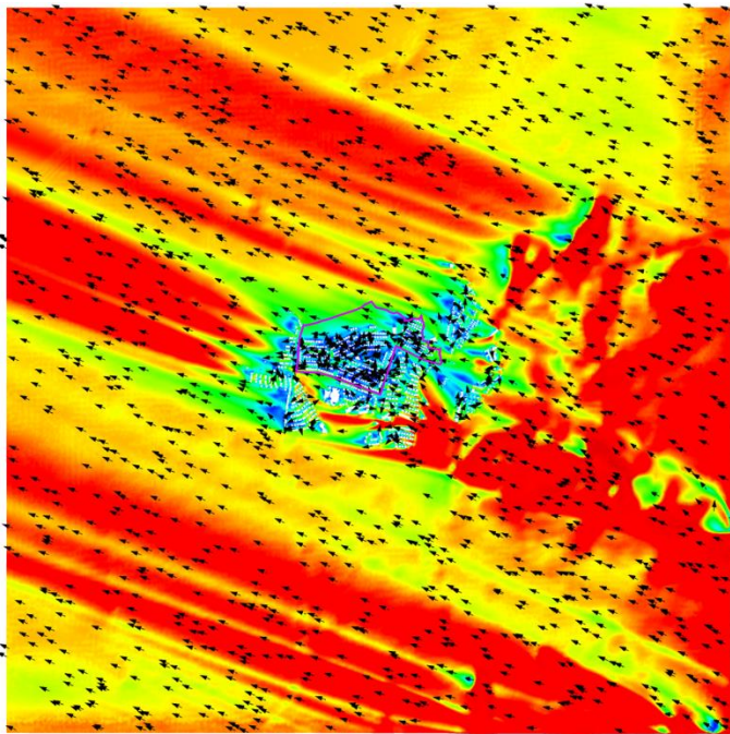
Figure 18 VR Vector Plot of Whole Domain at Pedestrian Level under ESE Wind for Baseline Scheme
