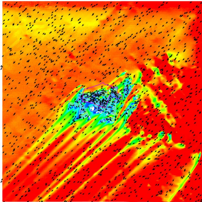
Figure 6 VR Vector Plot of Whole Domain at Pedestrian Level under NE Wind for Baseline Scheme
