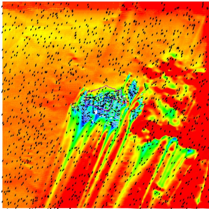
Figure 4 VR Vector Plot of Whole Domain at Pedestrian Level under NNE Wind for Proposed Scheme
