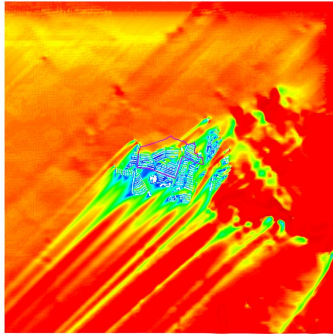
Figure 5 VR Contour Plot of Whole Domain at Pedestrian Level under NE Wind for Baseline Scheme
