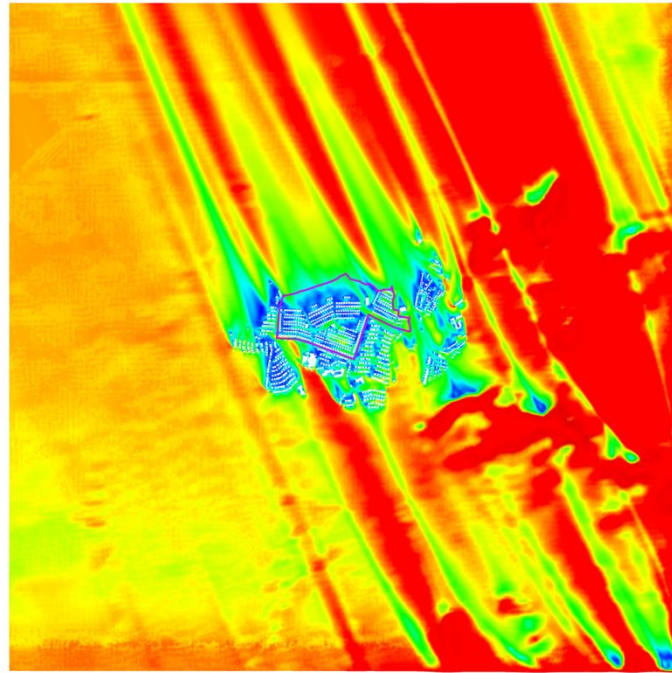
Figure 25 VR Contour Plot of Whole Domain at Pedestrian Level under SSE Wind for Baseline Scheme
