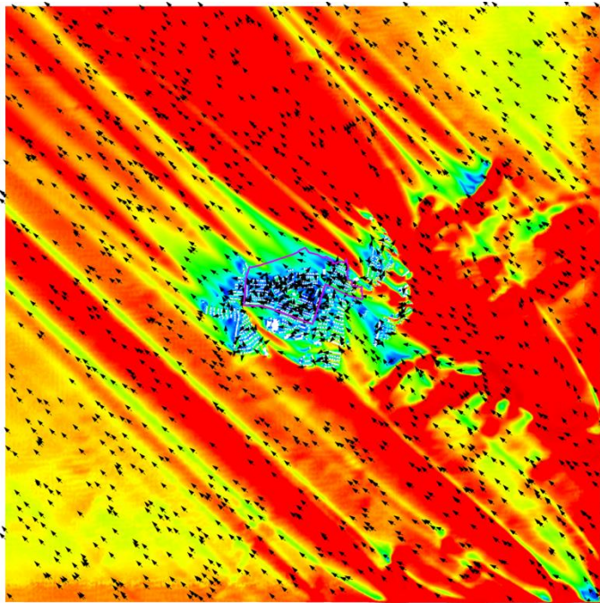
Figure 22 VR Vector Plot of Whole Domain at Pedestrian Level under SE Wind for Baseline Scheme
