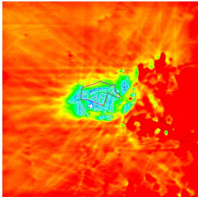
Figure 42 Annual Weighted Average VR Contour Plot of Whole Domain at Pedestrian Level for Proposed Scheme
