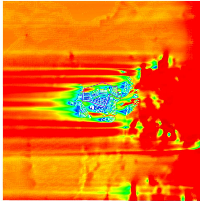
Figure 13 VR Contour Plot of Whole Domain at Pedestrian Level under E Wind for Baseline Scheme
