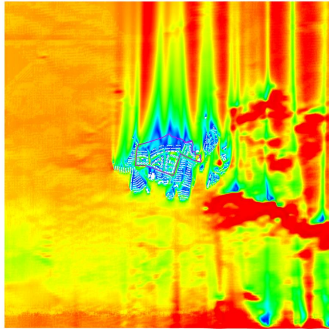
Figure 31 VR Contour Plot of Whole Domain at Pedestrian Level under S Wind for Proposed Scheme
