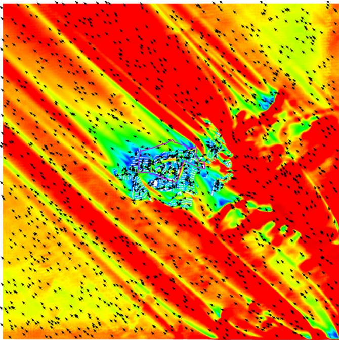
Figure 24 VR Vector Plot of Whole Domain at Pedestrian Level under SE Wind for Proposed Scheme
